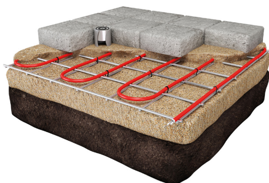
Installation in sand bed under paving stones
