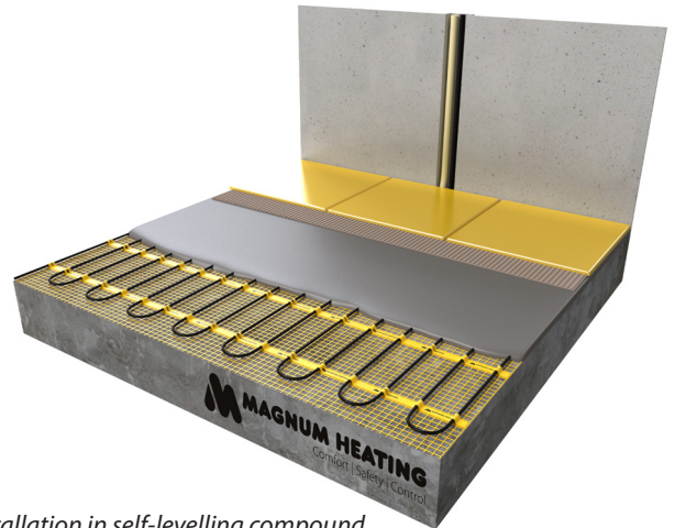
Installation in self-levelling compound
