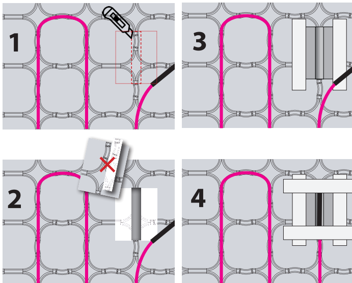
Example of the installation for Heatboard E Cable
